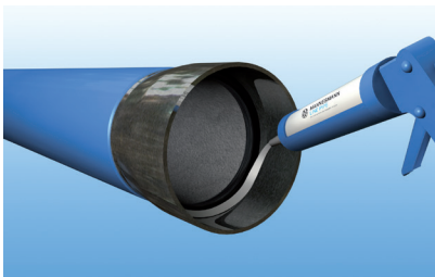
Sealant application
