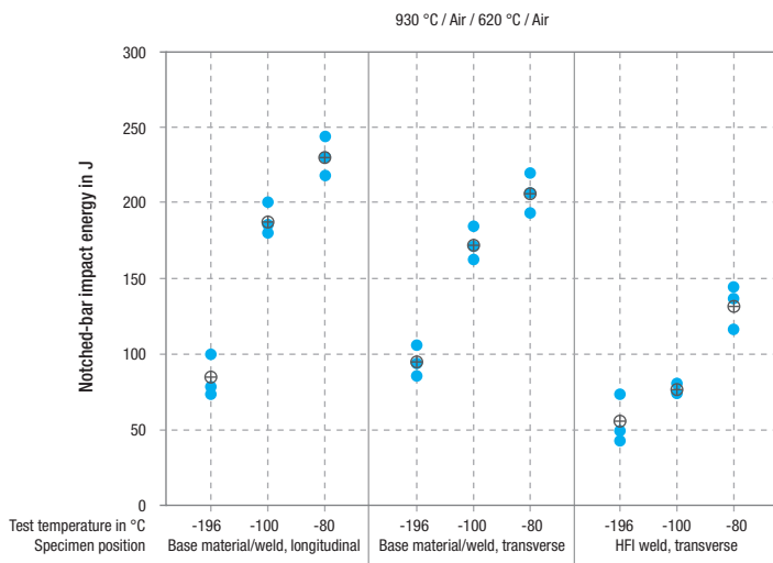
Figure 1: Charpy-V test results (full-size specimen after Q & T) as a function of test temperature and specimen position
