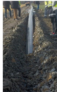
Installation of a high-pressure gas pipeline using the plowing technique
