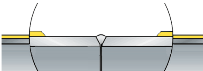
Butt-weld joint
